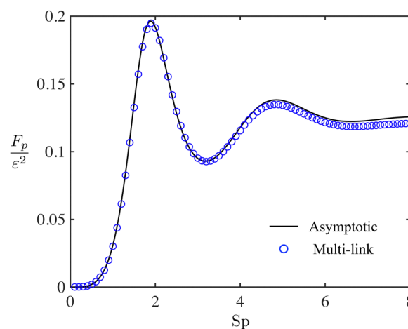
Fig. 6 The propulsive thrust F_p/\varepsilon^2 generated by an elastic filament oscillated harmonically at one end as a function of the sperm number Sp with \varepsilon = 0.1 . Numerical results from the multi-link model with N = 50 (blue circles) display satisfactory agreements with previous asymptotic results based on a continuum description of the elastic filament 36 (black solid line).
