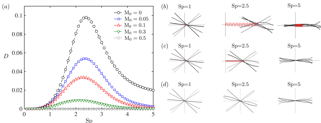
Fig. 3 Propulsion characteristics of the elastic filament with magnetic moments of same polarity. (a) The dimensionless displacement of the filament D in a single cycle as a function of the sperm number, Sp , at varying levels of relative magnetic strength M_0 . Panels (b)–(d): the shape of the filament at different time instants in a cycle (the color of the filament turns from light to dark as time proceeds) at different Sp for (b) M_0 = 0 , (c) M_0 = 0.05 , and (d) M_0 = 0.5 . Here the red lines display the trajectories of the mid-point of the filament from their initial positions represented by the vertical black lines over 10 cycles.
