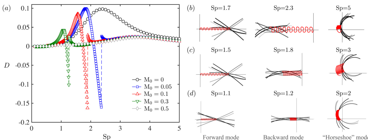
Fig. 4 Propulsion characteristics of the elastic filament with magnetic moments of opposite polarity. (a) The dimensionless displacement of the filament D in a single cycle as a function of the sperm number, Sp , at varying levels of relative magnetic strength M_0 . Panels (b)–(d): the shape of the filament at different time instants in a cycle (the color of the filament turns from light to dark as time proceeds) at different Sp for (b) M_0 = 0.05 , (c) M_0 = 0.1 , and (d) M_0 = 0.3 . Here the red lines display the trajectories of the mid-point of the filament from their initial positions represented by the vertical black lines over 10 cycles.
