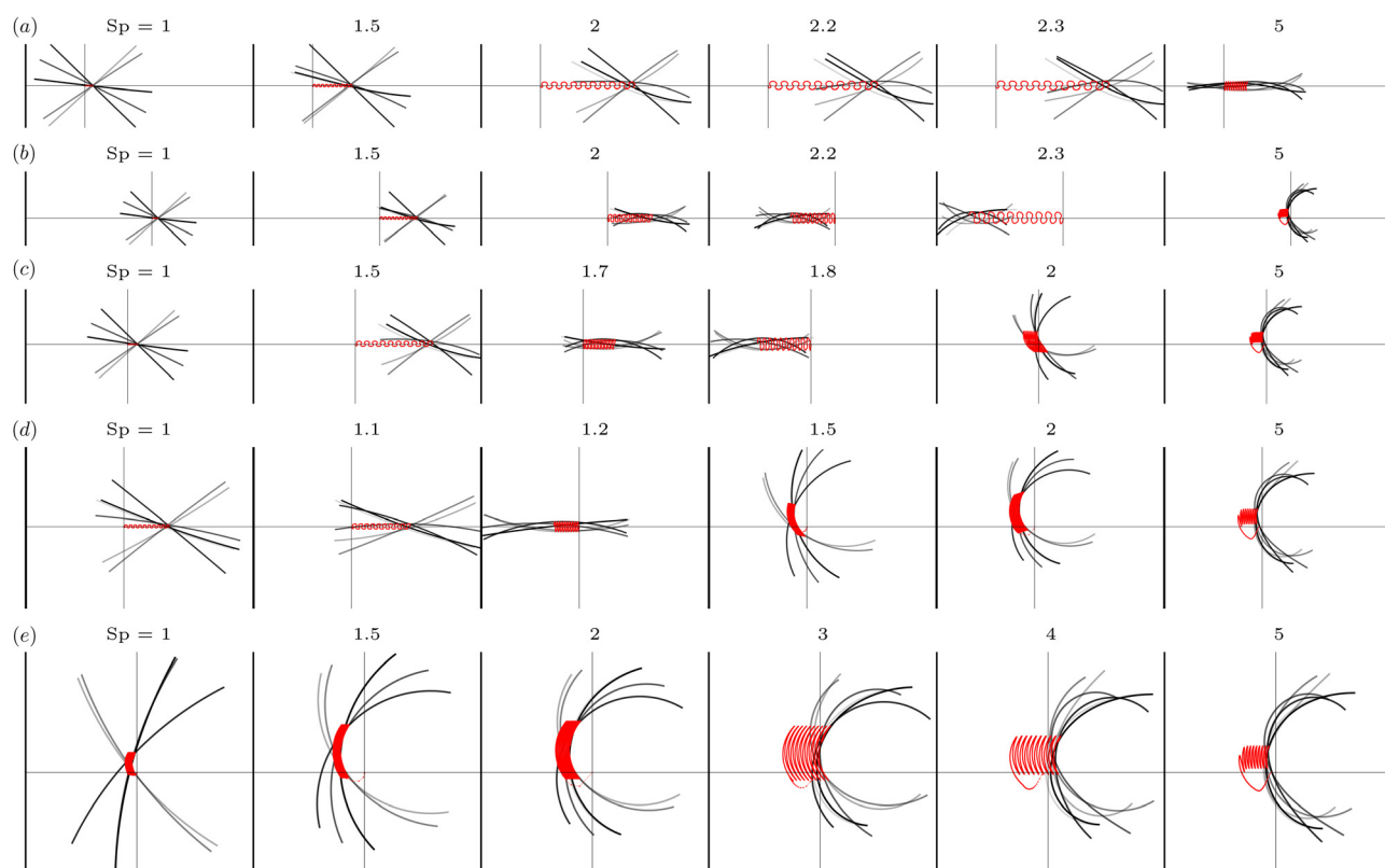
Fig. 5 Deformation of the filament with magnetic moments of opposite polarity. The shape of the filament at different time instants in a cycle (the color of the filament turns from light to dark as time proceeds) at different Sp for (a) M_0 = 0 , (b) M_0 = 0.05 , (c) M_0 = 0.1 , (d) M_0 = 0.3 , and (e) M_0 = 0.5 . Here the red lines display the trajectories of the mid-point of the filament from their initial positions represented by the vertical black lines over 10 cycles.
